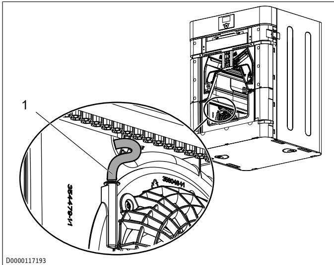
1 Pressure hose
