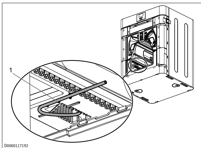
1 Pressure hose retainer
