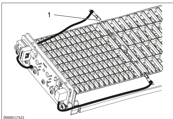
1 Safety assembly
